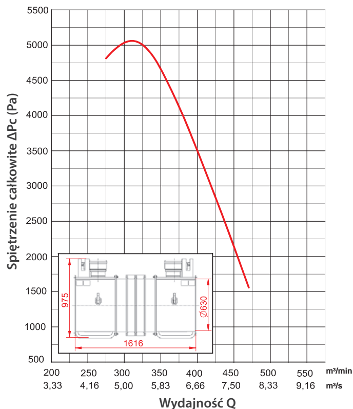
Charakterystyka wentylatora GWE-630B/2x18,5
